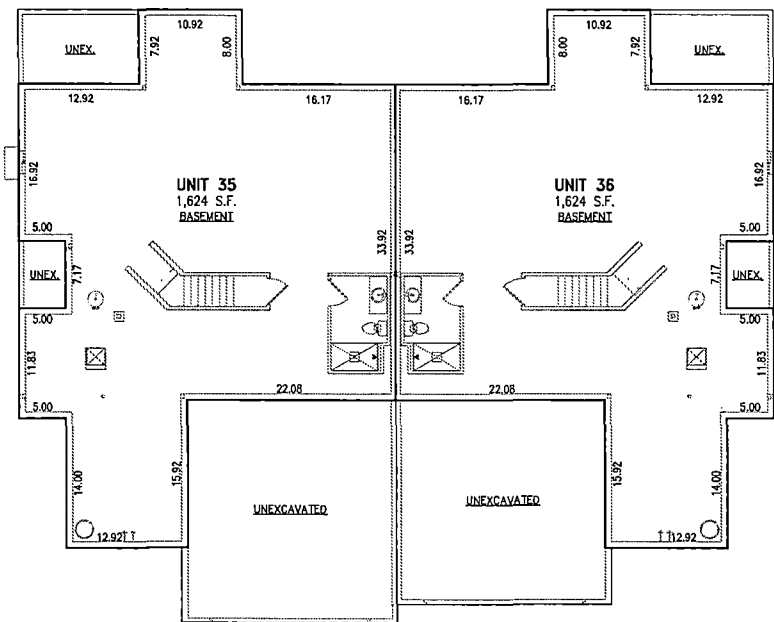
BUILDING 18 FOUNDATION PLAN
