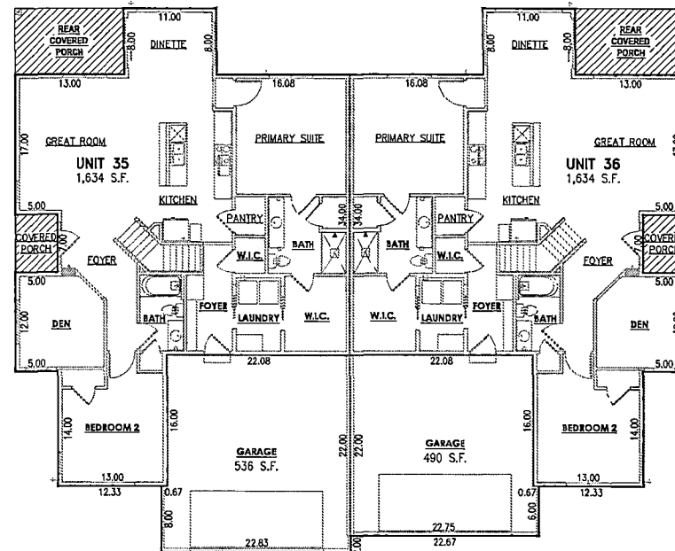
BUILDING 18 FIRST FLOOR PLAN
