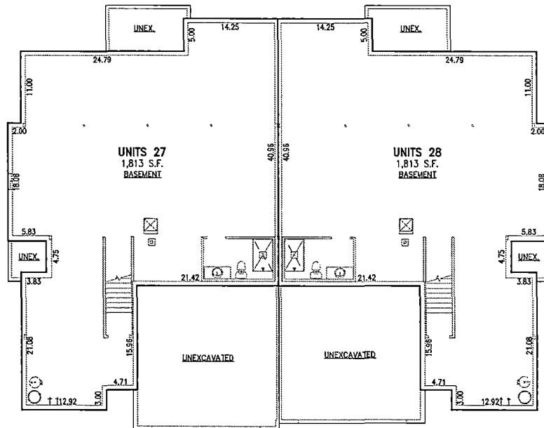
BUILDING 14 FOUNDATION PLAN
