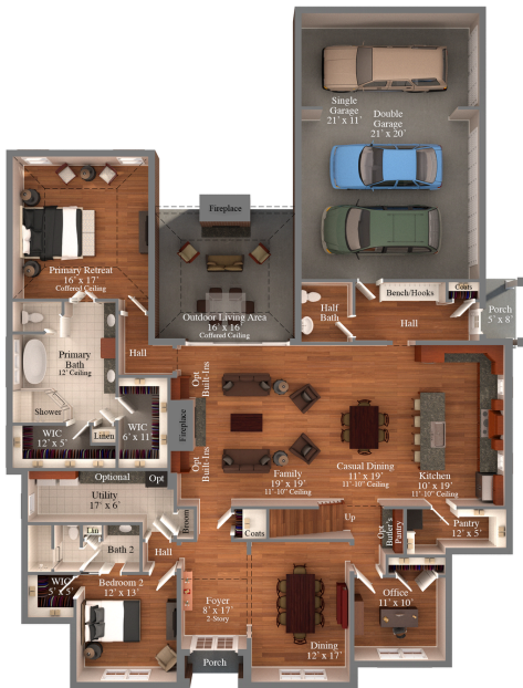
First Floor: 10' Ceilings unless noted
